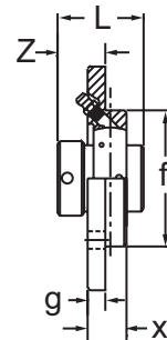
UGME 200 Type Eccentric Collar Locking
