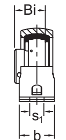
BPR 200 Type Set-Screw Locking
