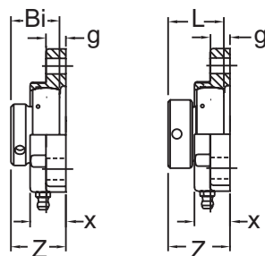
BTM 200 Type Set-Screw Locking
